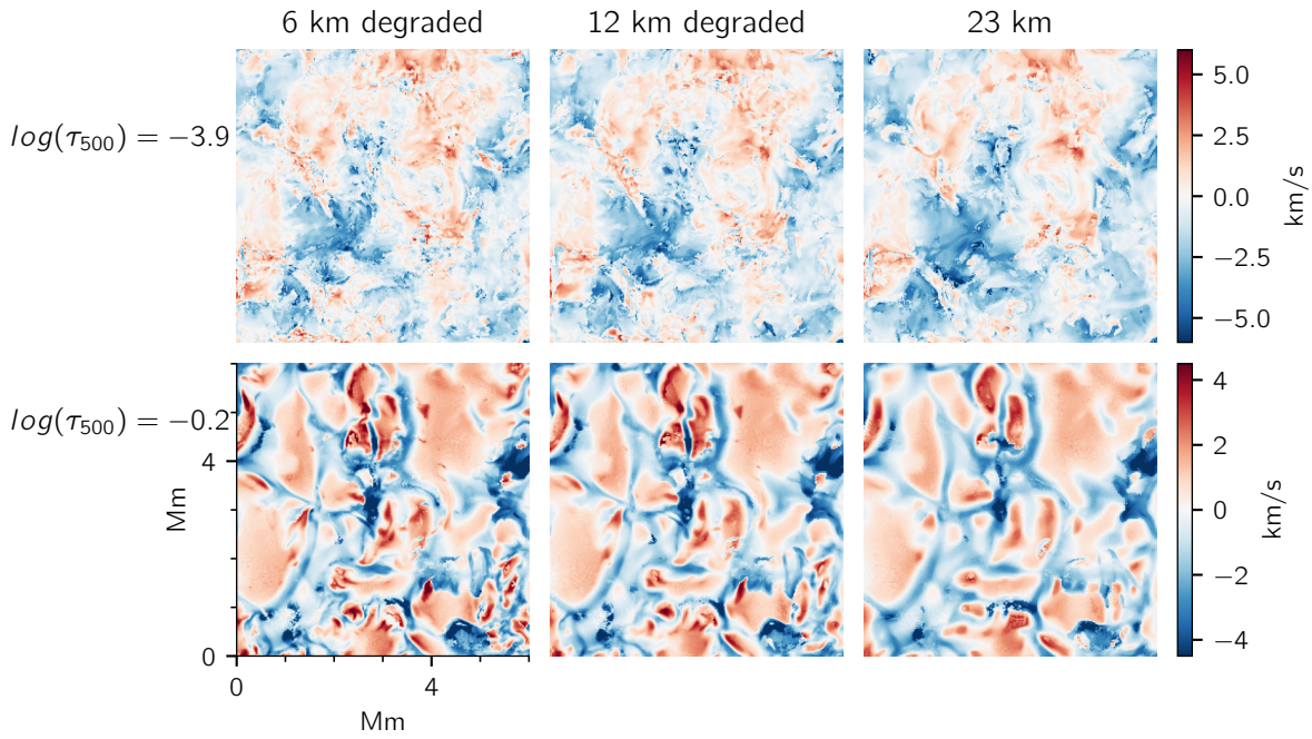
Fig. 8. Retrieved line-of-sight velocities from the inversions of the (degraded) spectra, taken at the heights \log(\tau_{500}) = -3.9 (top) and \log(\tau_{500}) = -0.2 (bottom), corresponding to the lower chromosphere and the photosphere respectively.
