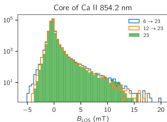
Fig. 7. Histograms of the inferred line-of-sight magnetic field strengths for the Ca II core after degradation to the common 23 km resolution, using the WFA-method Eq. 3. Note that here, as in Fig. 5, we include the whole horizontal extent of the simulation in the histograms, not only the quadrant shown in the colormaps elsewhere.
