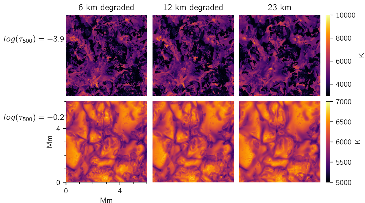
Fig. 10. Retrieved temperatures from the inversions of the (degraded) spectra, taken at the heights \log(\tau_{500}) = -3.9 (top) and \log(\tau_{500}) = -0.2 (bottom), corresponding to the lower chromosphere and the photosphere respectively.
