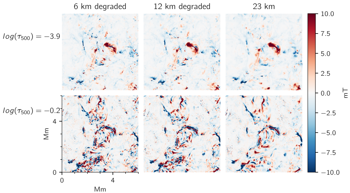
Fig. 9. Retrieved line-of-sight magnetic field strengths from the inversions of the (degraded) spectra, taken at the heights \log(\tau_{500}) = -3.9 (top) and \log(\tau_{500}) = -0.2 (bottom), corresponding to the lower chromosphere and the photosphere respectively.
