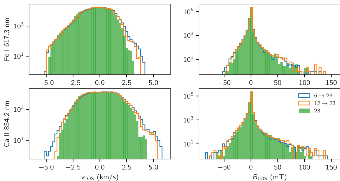
Fig. 5. Histograms of the inferred quantities using the COG-method on the whole line profile for Fe I 617.33 nm (top) and Ca II 854.209 nm (bottom). Note that here, as in Fig. 7, we include the whole field of view for the simulation in the histograms, not only the quadrant shown in the colormaps elsewhere.
